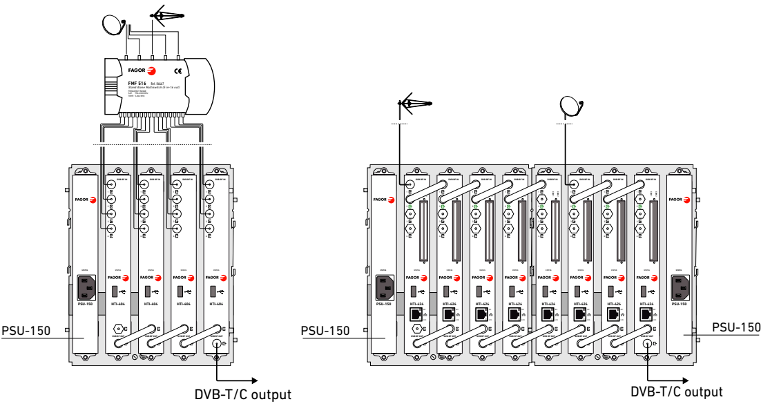
Installation example containing 4 HTI transmodulators + 1 PSU-150 power supply
